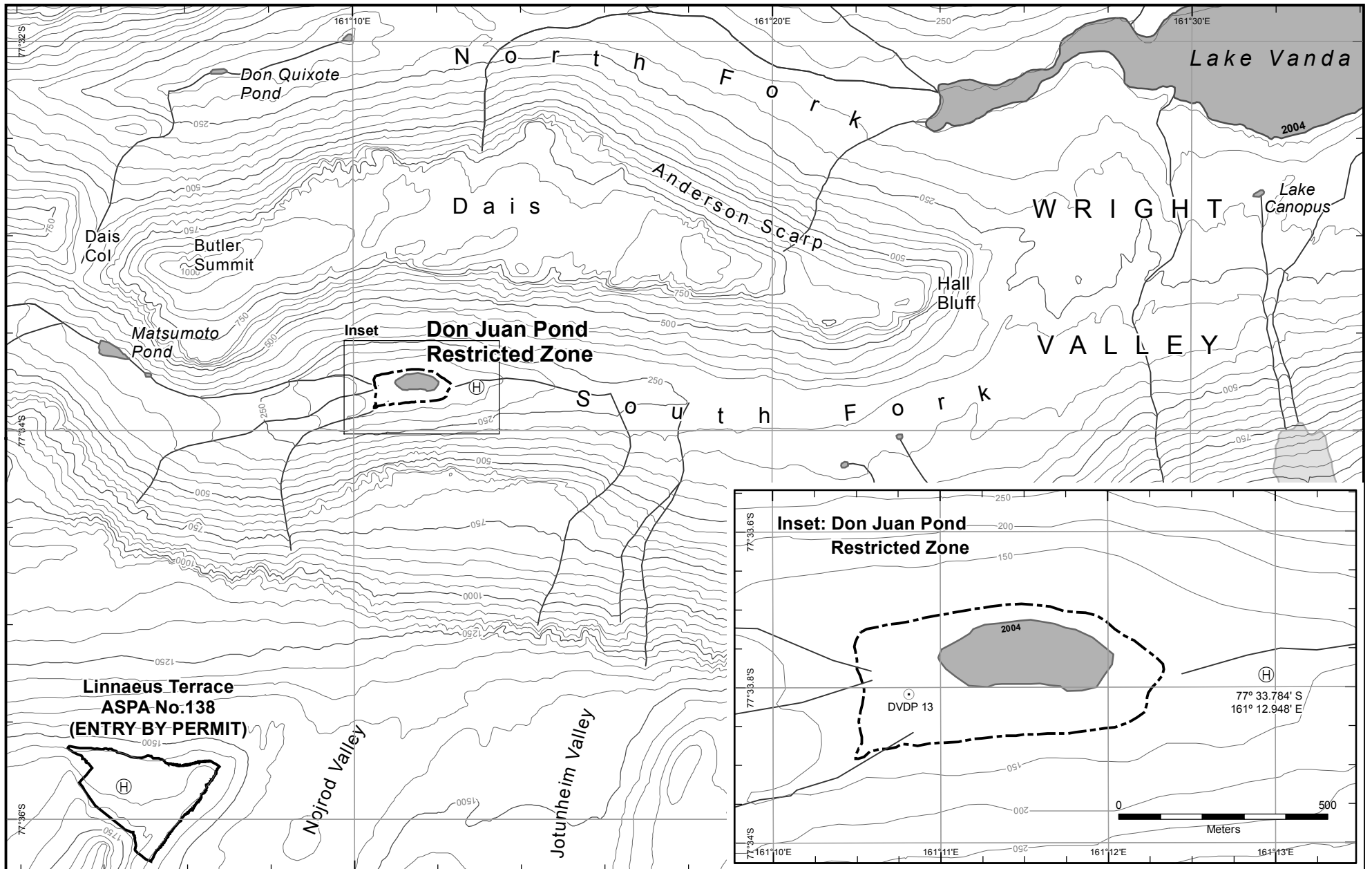
Map 18: Don Juan Pond, Wright Valley
